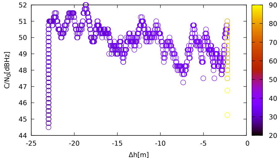
C/N 0 vs height (JavadVS (down) for R18 at L1)
