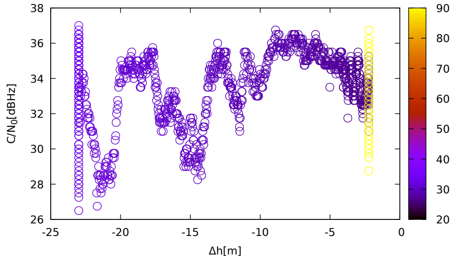
C/N 0 vs height (JavadVS (down) for R20 at L1)
