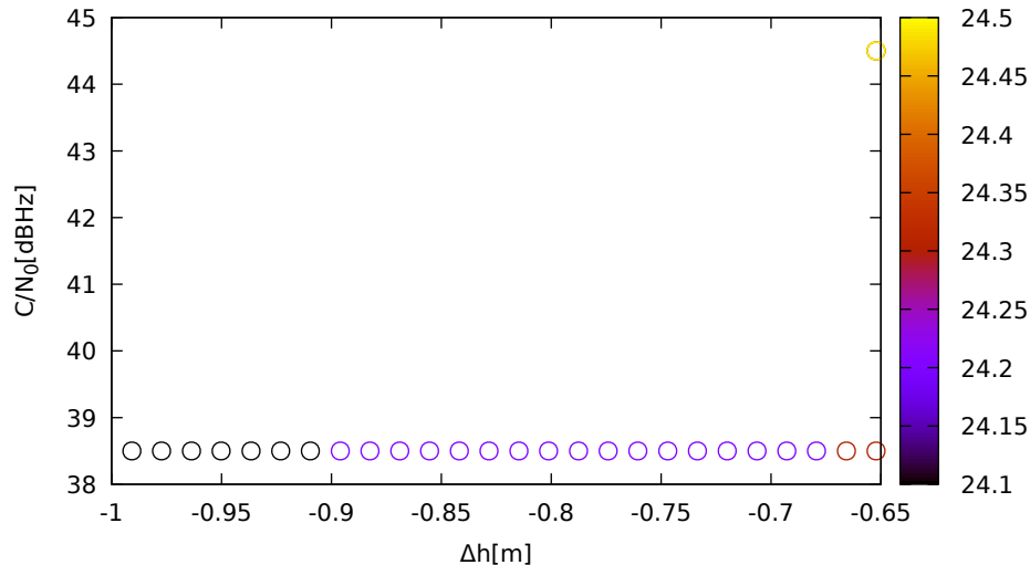
C/N 0 vs height (LeicaGS15 (down) for E01 at L1)
