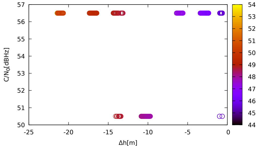
C/N 0 vs height (LeicaGS15 (down) for E12 at L1)
