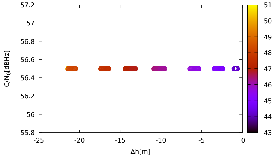
C/N 0 vs height (LeicaGS15 (down) for E24 at L1)
