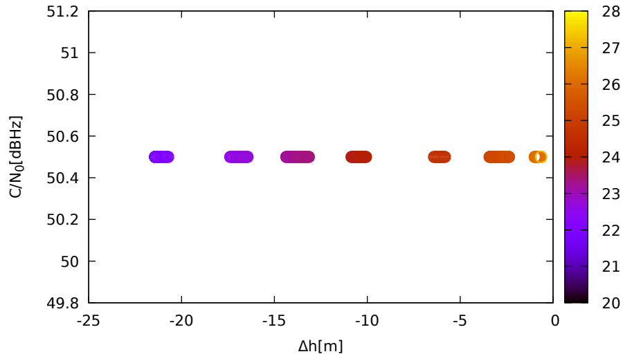
C/N 0 vs height (LeicaGS15 (down) for E26 at L1)
