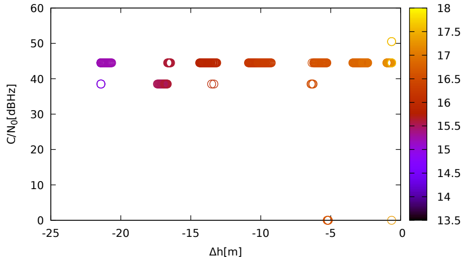
C/N 0 vs height (LeicaGS15 (down) for G05 at L1)
