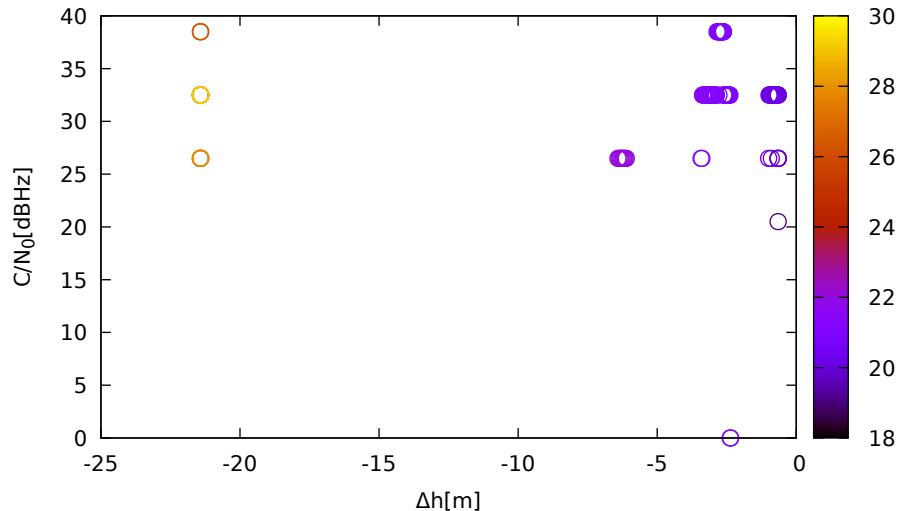
C/N 0 vs height (LeicaGS15 (down) for G16 at L1)
