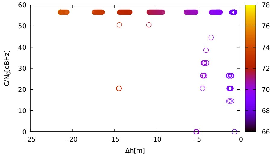
C/N 0 vs height (LeicaGS15 (down) for G18 at L1)
