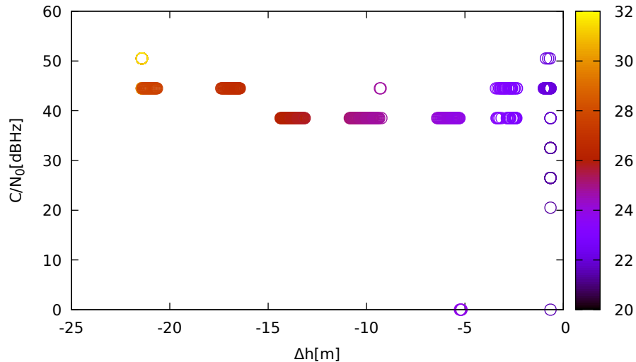
C/N 0 vs height (LeicaGS15 (down) for G21 at L1)
