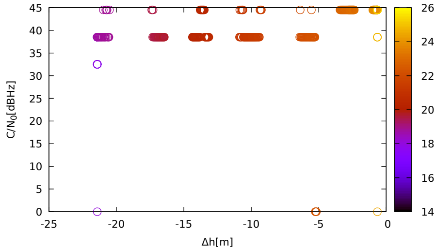
C/N 0 vs height (LeicaGS15 (down) for G25 at L1)
