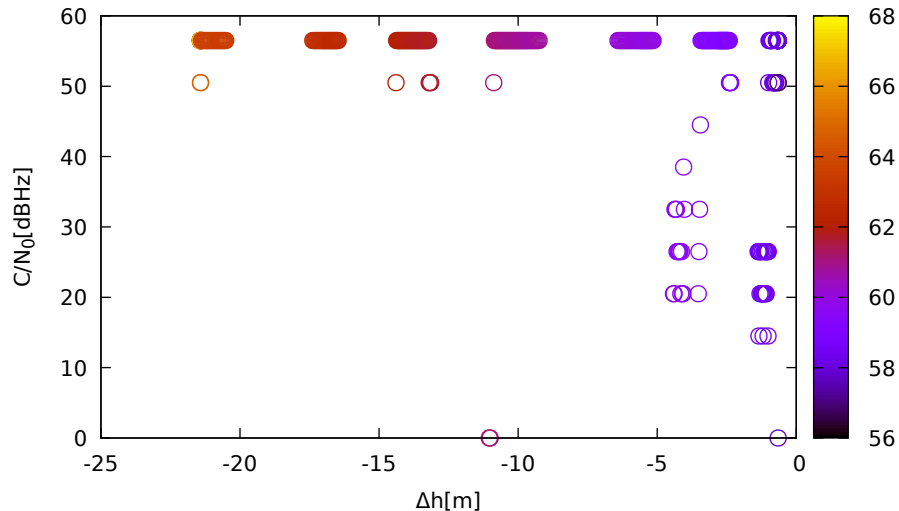
C/N 0 vs height (LeicaGS15 (down) for G26 at L1)
