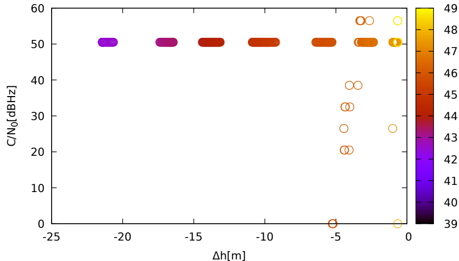
C/N 0 vs height (LeicaGS15 (down) for G29 at L1)
