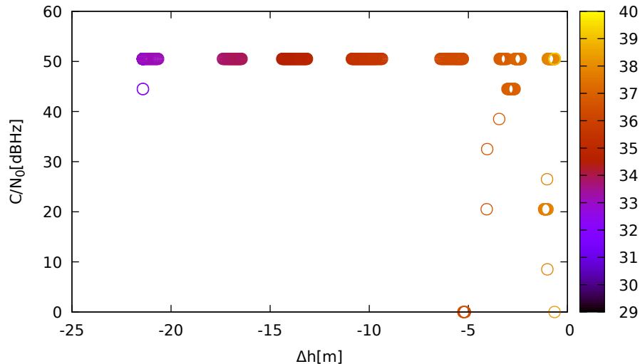
C/N 0 vs height (LeicaGS15 (down) for G31 at L1)
