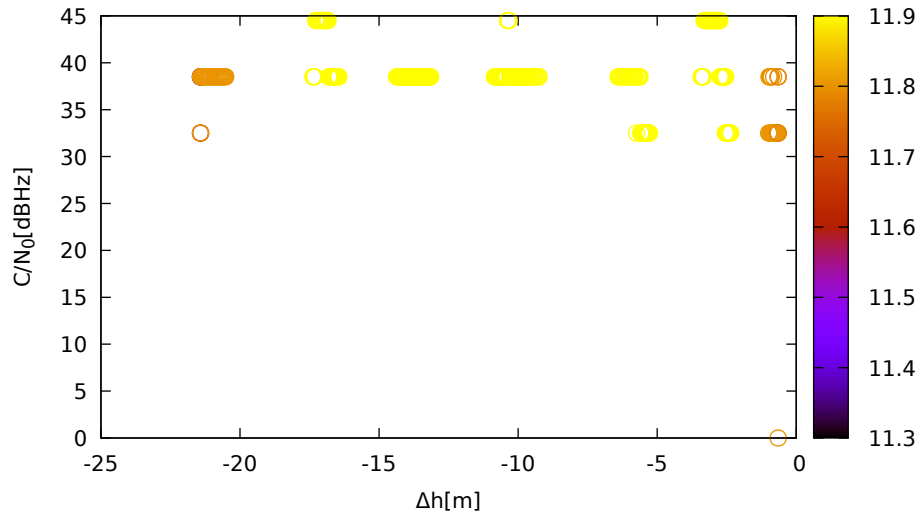
C/N 0 vs height (LeicaGS15 (down) for R02 at L1)
