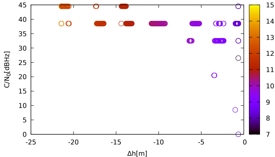
C/N 0 vs height (LeicaGS15 (down) for R03 at L1)
