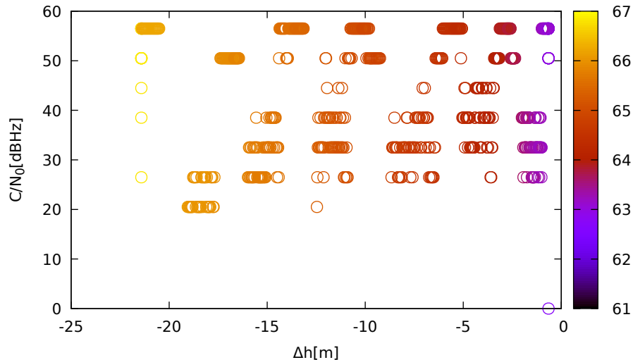
C/N 0 vs height (LeicaGS15 (down) for R09 at L1)
