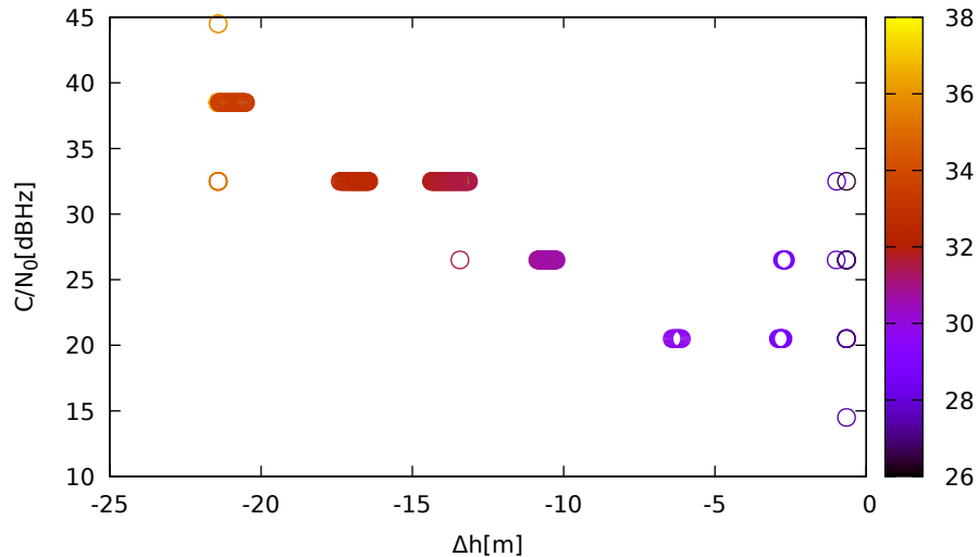
C/N 0 vs height (LeicaGS15 (down) for R10 at L1)
