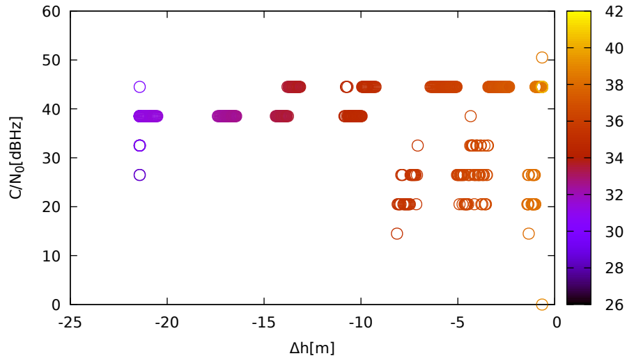
C/N 0 vs height (LeicaGS15 (down) for R16 at L1)
