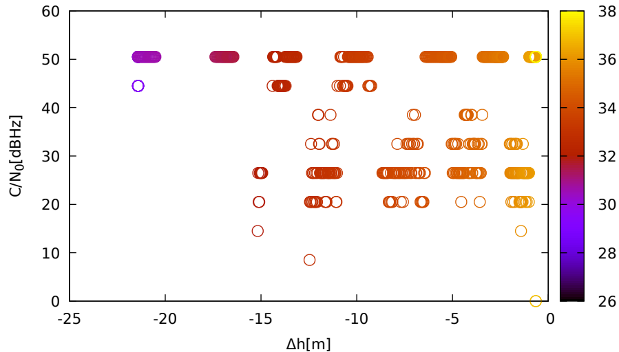
C/N 0 vs height (LeicaGS15 (down) for R18 at L1)
