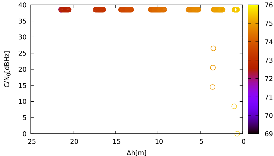
C/N 0 vs height (LeicaGS15 (down) for R19 at L1)
