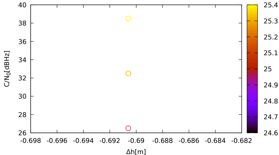
C/N 0 vs height (LeicaGS18 (down) for E01 at L1)
