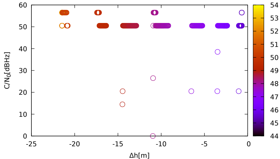
C/N 0 vs height (LeicaGS18 (down) for E12 at L1)
