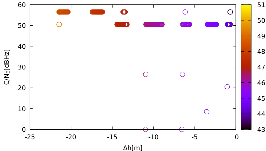
C/N 0 vs height (LeicaGS18 (down) for E24 at L1)
