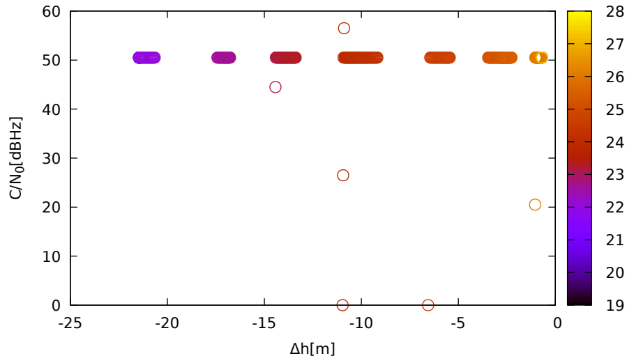
C/N 0 vs height (LeicaGS18 (down) for E26 at L1)
