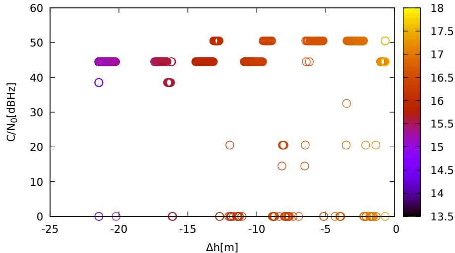
C/N 0 vs height (LeicaGS18 (down) for G05 at L1)
