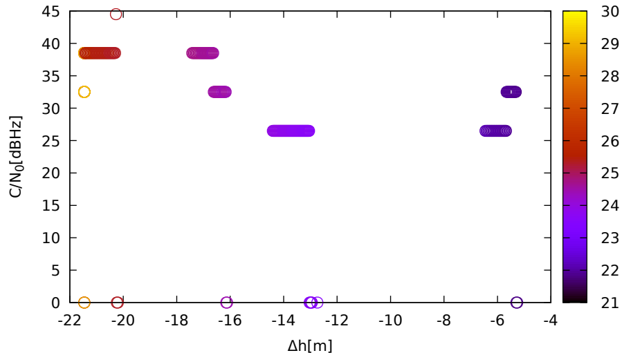
C/N 0 vs height (LeicaGS18 (down) for G16 at L1)
