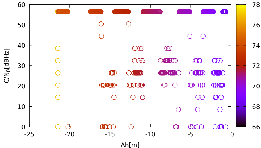
C/N 0 vs height (LeicaGS18 (down) for G18 at L1)
