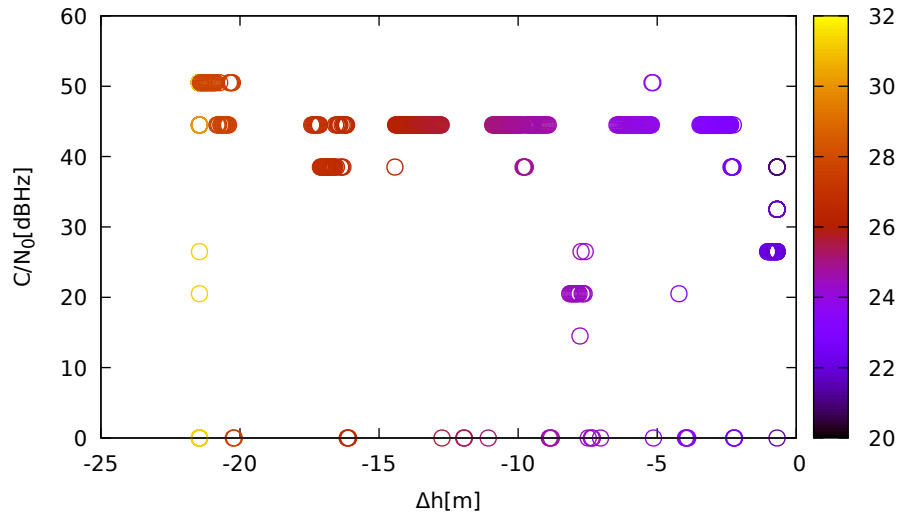
C/N 0 vs height (LeicaGS18 (down) for G21 at L1)
