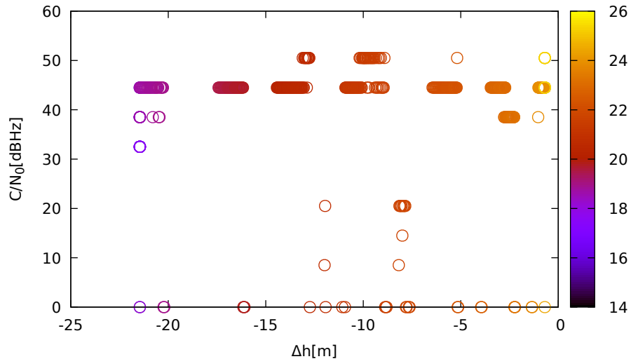
C/N 0 vs height (LeicaGS18 (down) for G25 at L1)
