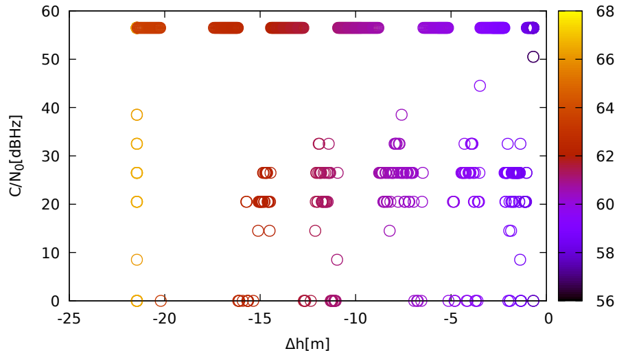
C/N 0 vs height (LeicaGS18 (down) for G26 at L1)
