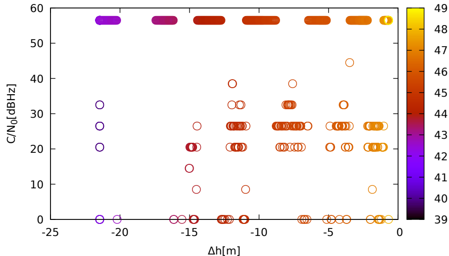
C/N 0 vs height (LeicaGS18 (down) for G29 at L1)
