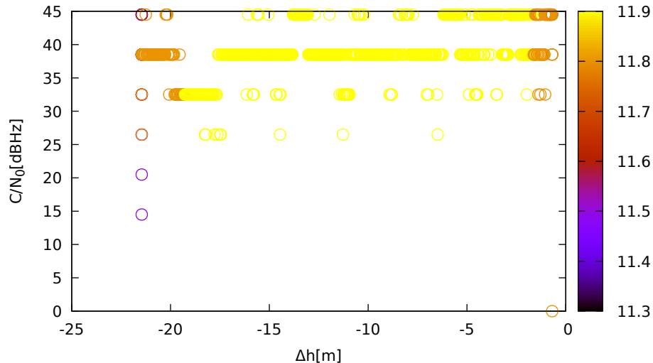
C/N 0 vs height (LeicaGS18 (down) for R02 at L1)
