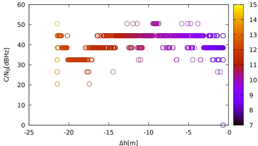
C/N 0 vs height (LeicaGS18 (down) for R03 at L1)
