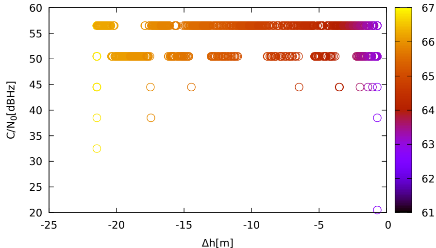
C/N 0 vs height (LeicaGS18 (down) for R09 at L1)
