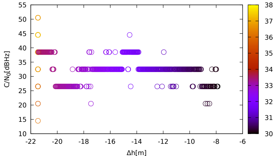
C/N 0 vs height (LeicaGS18 (down) for R10 at L1)
