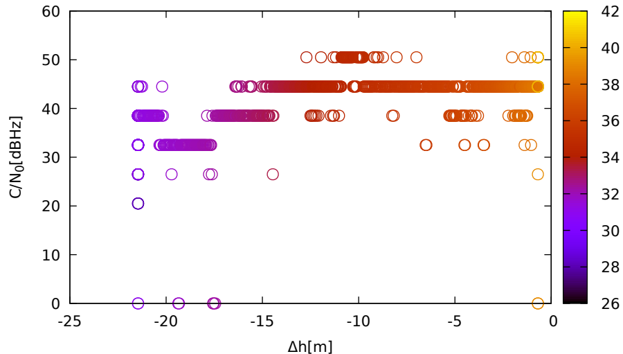
C/N 0 vs height (LeicaGS18 (down) for R16 at L1)
