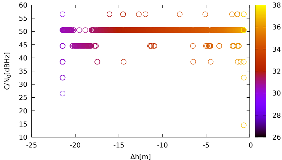
C/N 0 vs height (LeicaGS18 (down) for R18 at L1)
