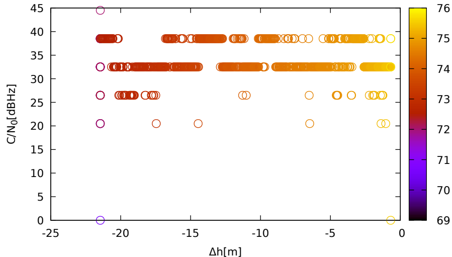
C/N 0 vs height (LeicaGS18 (down) for R19 at L1)
