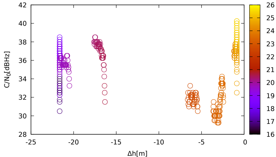
C/N 0 vs height (TrimbleR10 (down) for E01 at L1)
