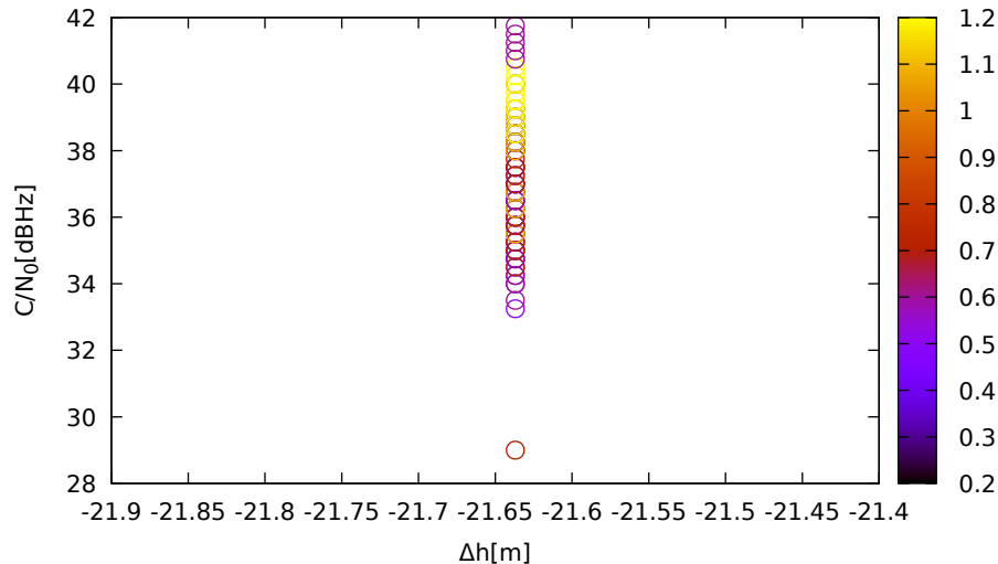
C/N 0 vs height (TrimbleR10 (down) for E07 at L1)
