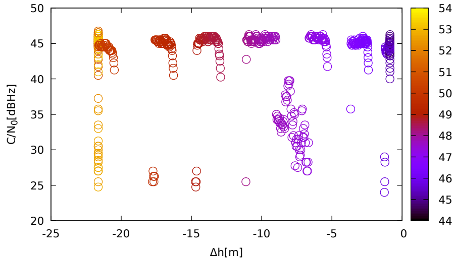
C/N 0 vs height (TrimbleR10 (down) for E12 at L1)
