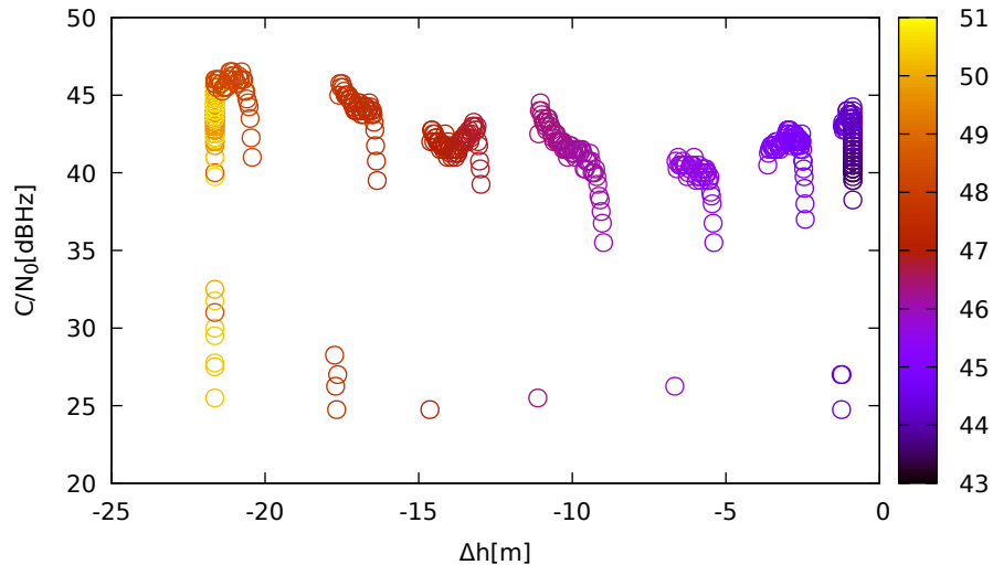
C/N 0 vs height (TrimbleR10 (down) for E24 at L1)
