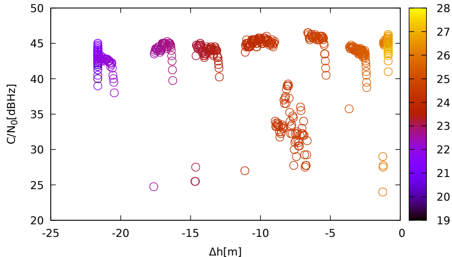
C/N 0 vs height (TrimbleR10 (down) for E26 at L1)
