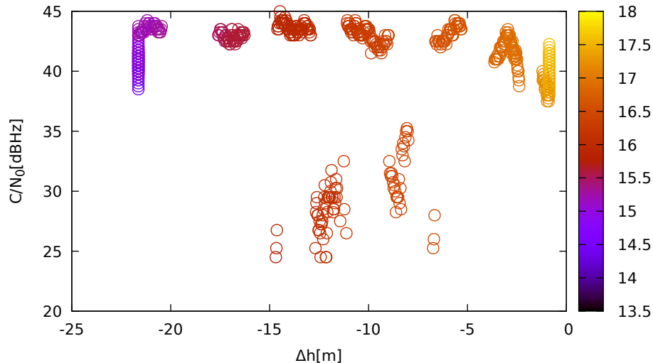
C/N 0 vs height (TrimbleR10 (down) for G05 at L1)
