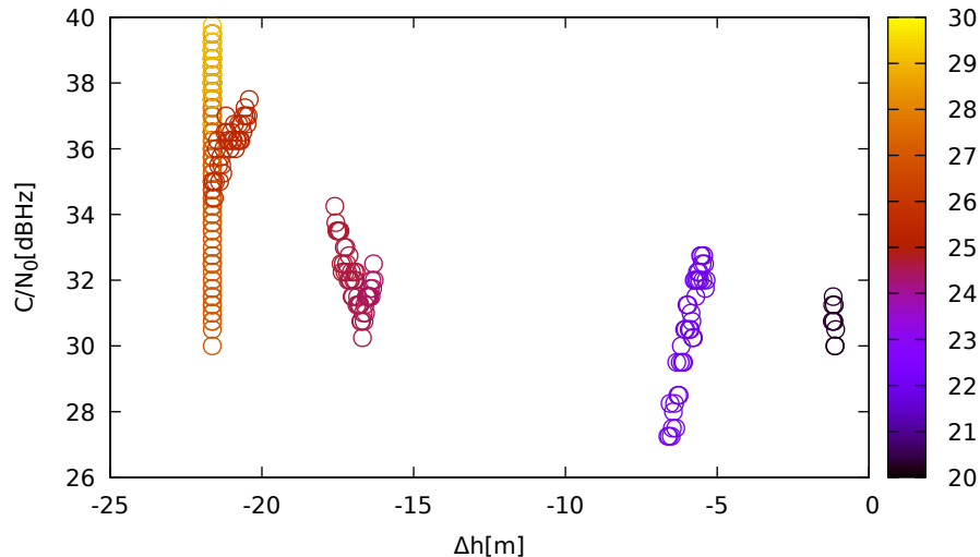
C/N 0 vs height (TrimbleR10 (down) for G16 at L1)
