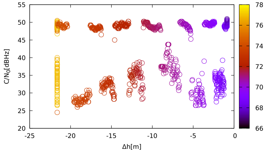
C/N 0 vs height (TrimbleR10 (down) for G18 at L1)
