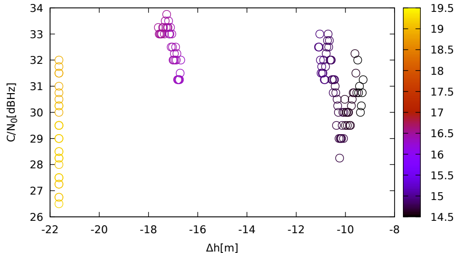
C/N 0 vs height (TrimbleR10 (down) for G20 at L1)
