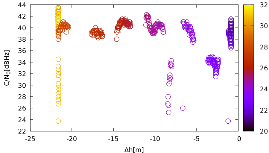
C/N 0 vs height (TrimbleR10 (down) for G21 at L1)
