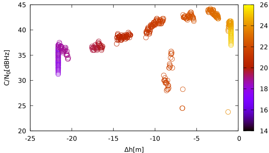
C/N 0 vs height (TrimbleR10 (down) for G25 at L1)
